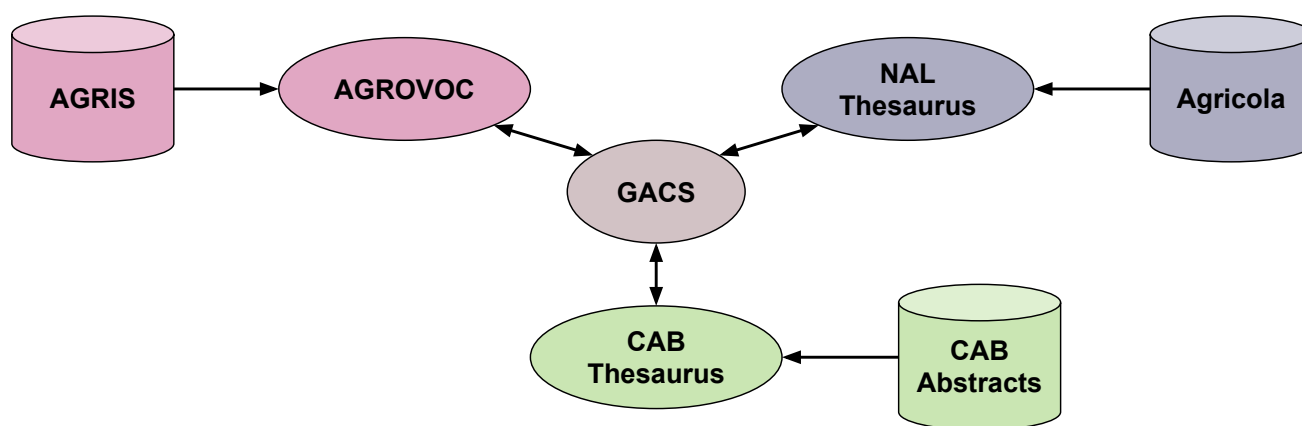
Figure 3: Overview of GACS Beta, its relationship to the participating thesauri via mappings that form a hub-and-spoke model, and the main publication databases currently referencing the thesauri.
