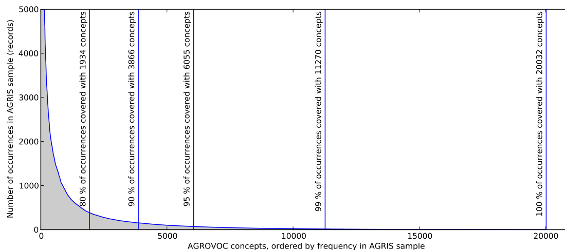
Figure 2: Long tail distribution of AGROVOC concepts in the AGRIS database.
