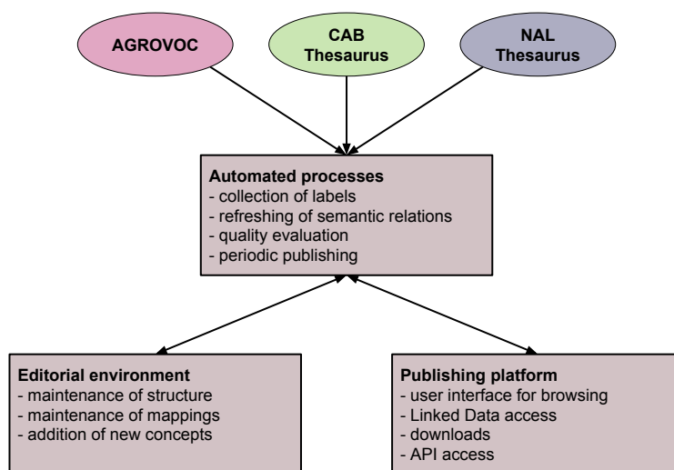
Figure 4: Overview of GACS technical infrastructure
