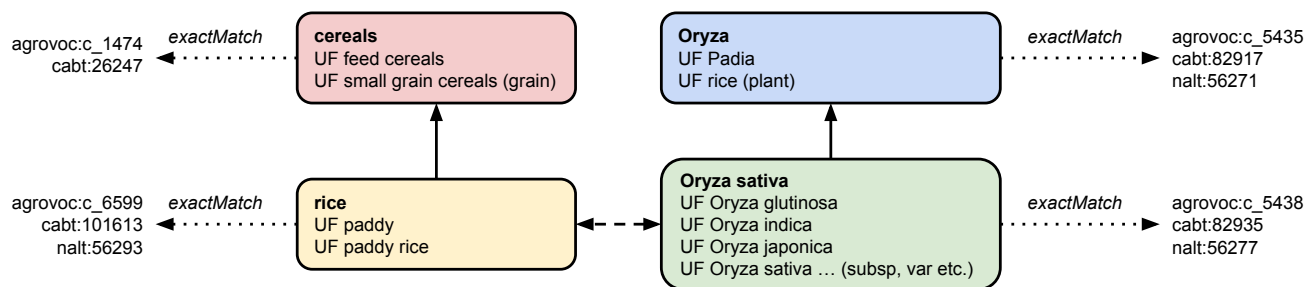
Figure 7: Modeling of rice-related concepts in GACS.
